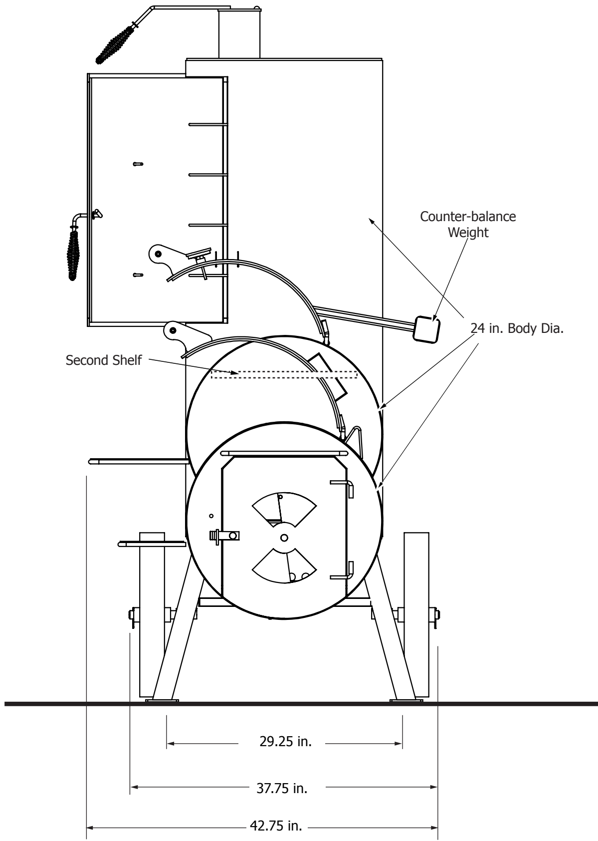
Durango 24" Smoker _ Firebox End View
