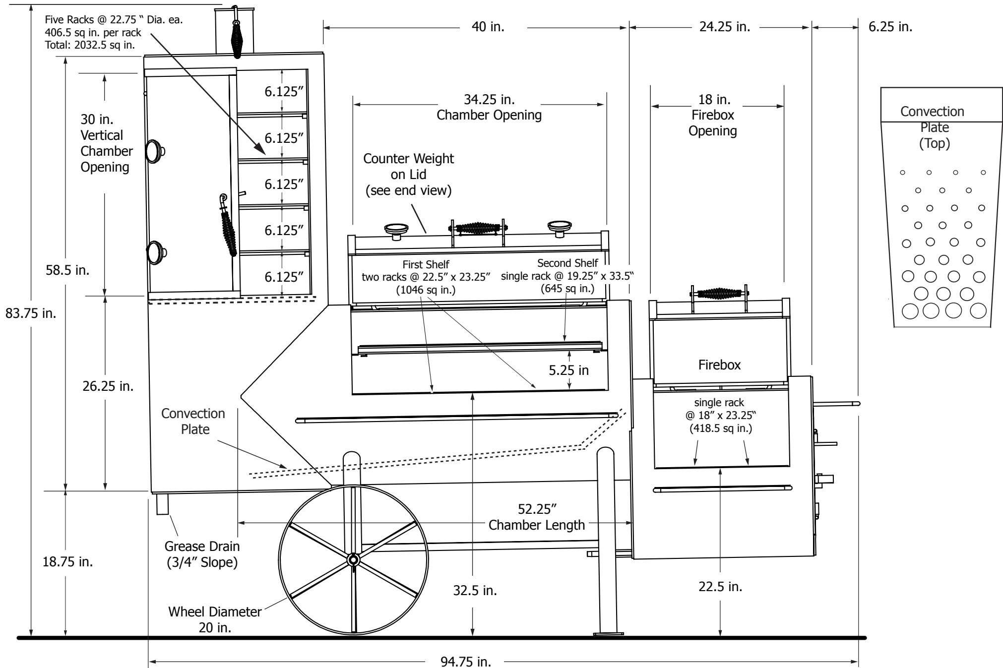
Durango 24" Smoker _ Front View
